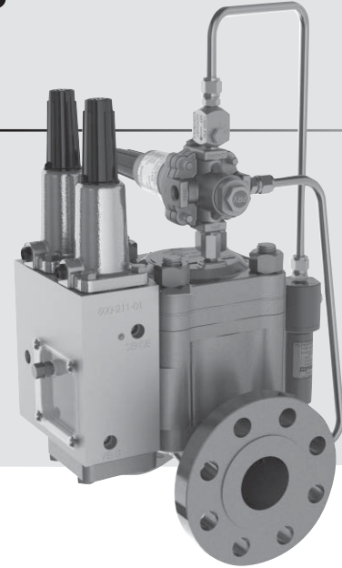
Flowgrid® Regulator with Integral Shutoff Valve, Series 60 Dual Function Controller, optional Series 20 Pilot, Type 24 Restrictor and Type 30 Filter.
